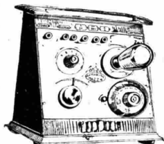
MONODINA ad 1 valvola
